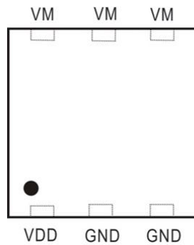
DFN2x2-6L
