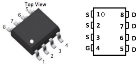
SOP-8 SES8619AG
